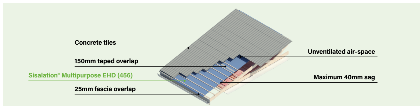
Figure 2: Low pitched residential tiled roof
